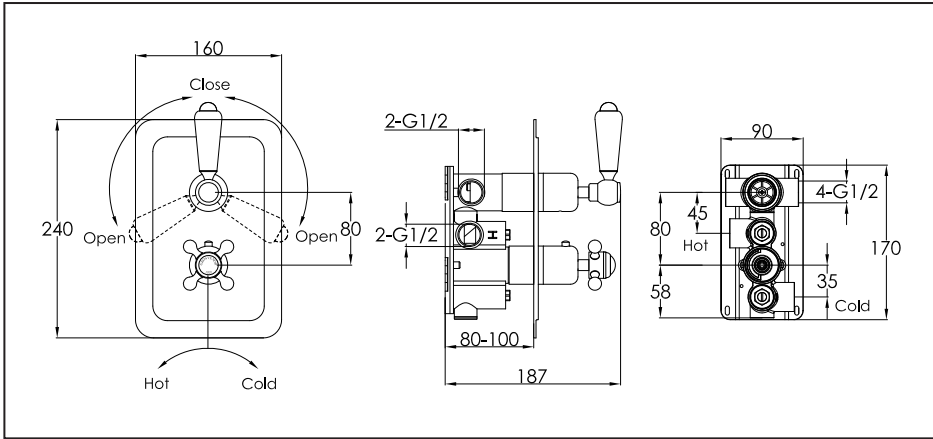
Dimension Drawing
