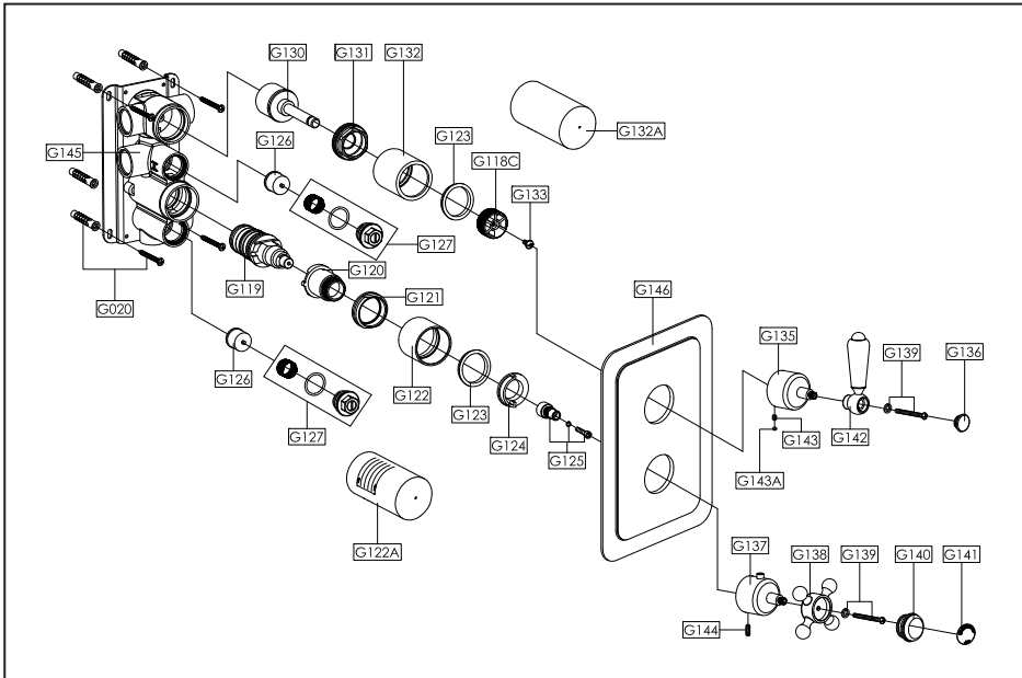
Explosive drawing
