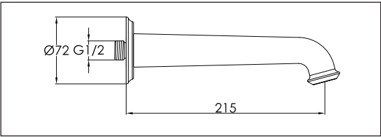
Dimension Drawing
